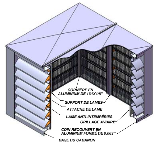
*CI-HAUT CABANON A COINS RECOUVERTS (BOX)
