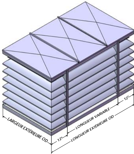
COINS RECOUVERTS *STANDARD PH-2625B
